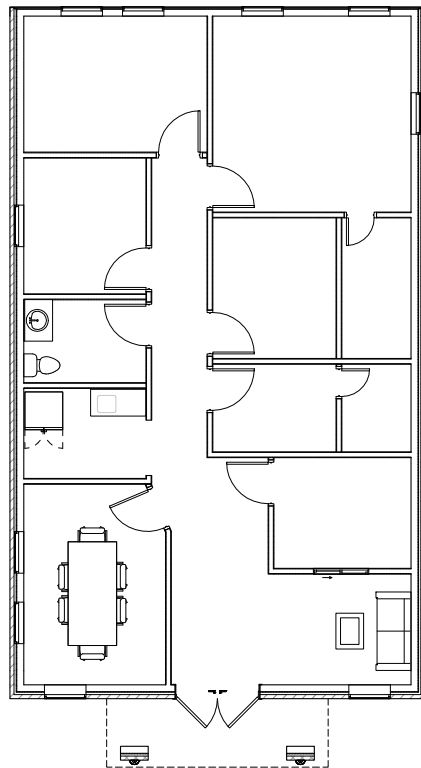
FOUNDATION PLAN - TYP. 1-10 RE: A 2.0-1 | 1/4" = 1'-0"
